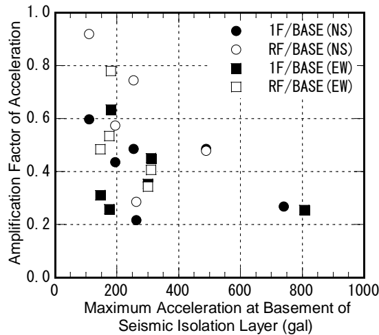
Figure 1 - Amplification Factor of Observed Acceleration of Seismic Isolated Buildings
